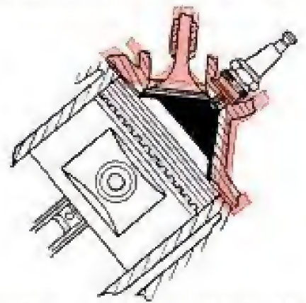
BUICK also redesigned its combustion chamber to add power. Red sketch shows 1953 design for comparison
